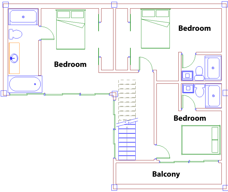
Floor 2
